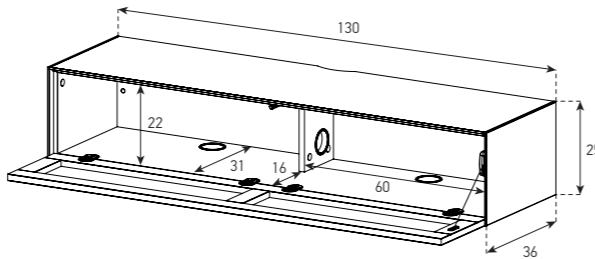
ED 66-TS (WITH CABLE MANAGEMENT)
