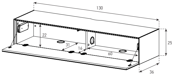
ED 66-F (WITH CABLE MANAGEMENT)
